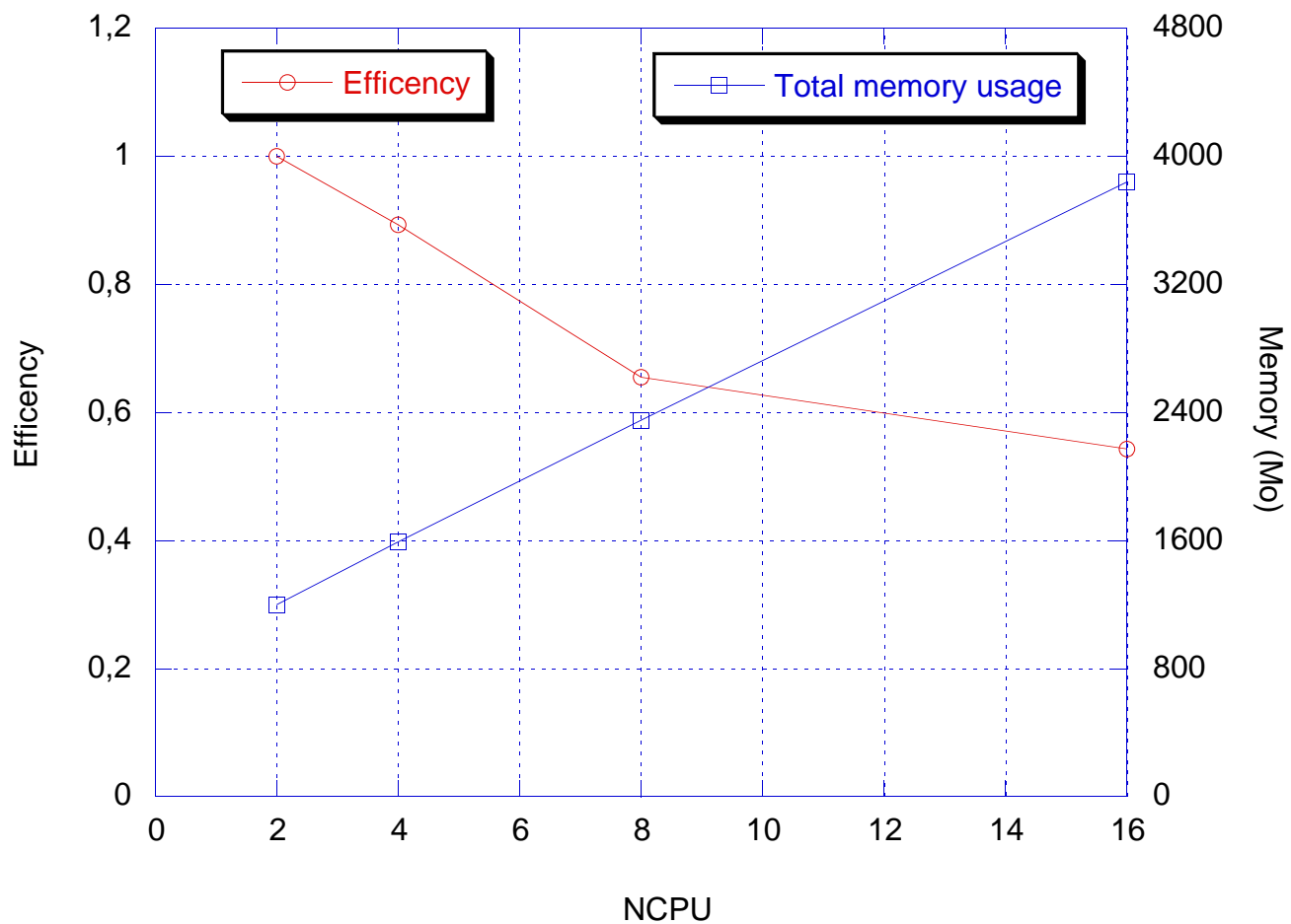
Lapw1_MPI (Matrix 5900)
